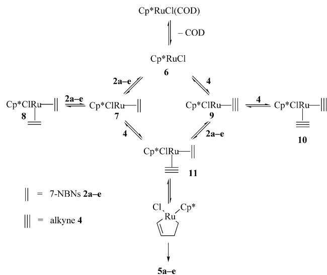
Scheme 2. The proposed mechanism for a Ru II -catalyzed [2+2] cycloaddition.
