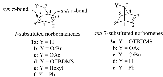
Figure 1. 7-Substituted norbornadienes and anti 7-substituted norbornenes.
